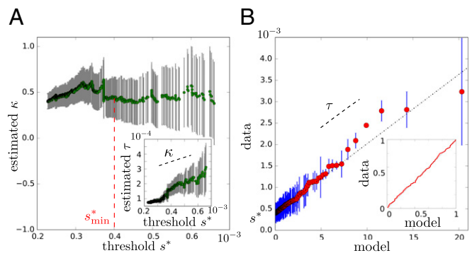
Fig. 4. Extreme value analysis by the point over threshold approach. (A) Values of the inferred parameter \hat{\kappa}(s^*) from selectivity s_i > s^* as a function of the threshold s^* . The inference is made by maximum likelihood, and the error bars indicate 95% confidence intervals. (A, Inset ) Similarly for \hat{\tau}(s^*) , the second parameter of the model, which is estimated jointly to \kappa(s^*) . For sufficiently large s^* , s^* > s_{\min}^* , \kappa(s^*) should be constant, and \hat{\tau}(s^*) should increase linearly with slope \kappa(s^*) . These relations are observed here for s_{\min}^* \simeq 4 \times 10^{-4} (red dotted line) with \kappa = 0.45 \pm 0.22 and \tau = 1.6 \times 10^{-4} \pm 10^{-5} ; \kappa = 0 can be excluded by likelihood ratio test with a P value < 10^{-4} . (B) Q-Q plot representing the data s_i against predictions from the model based on the inferred value of \kappa only. A straight line is expected for a good fit with a slope and the y intercept given by the two other parameters \tau and s^* . (B, Inset ) The P-P plot comparing the empirical cumulative distributions from the data with the cumulative distribution from the inferred model, showing an excellent agreement. The data come from the selection of the S1 library against the PVP target as in Fig. 3A ( SI Appendix , Figs. S8–S10 shows similar analyses of the data shown in Fig. 3B–D).
